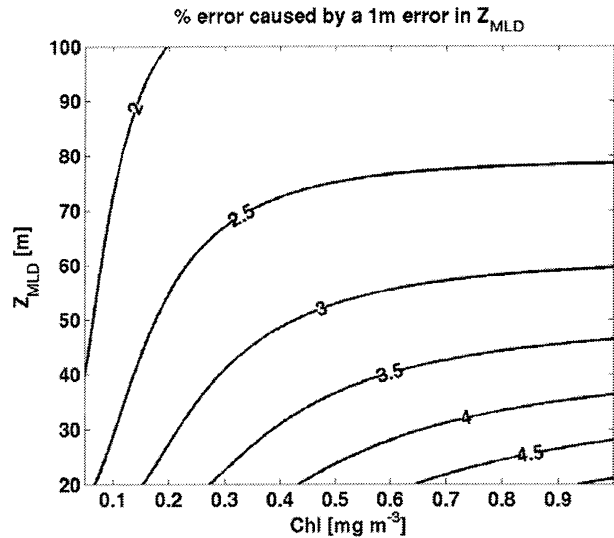
FIG. 7. The percentage error in biological heating (plotted as contours) caused by a 1-m error in the estimation of Z_{\text{MLD}} , plotted as a function of chlorophyll and Z_{\text{MLD}} . Biological heating is most sensitive to variability in Z_{\text{MLD}} at shallow mixed layer depths and high chlorophyll concentrations.
